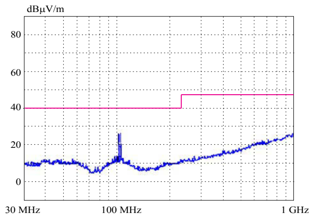
Fig. 3. The curve of LAN cables disturbing field – horizontal polarization
