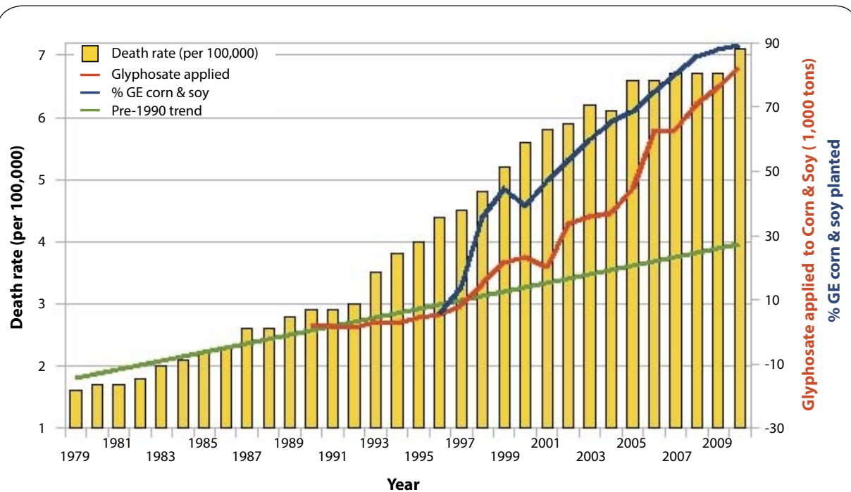
Figure 6. Deaths from Parkinson's disease (ICD G20 & 332.0) plotted against glyphosate use on corn & soy ( R=0.9006 , p \leq 5.063e-07 ) and %GE corn & soy planted ( R=0.9676 , p \leq 2.714e-06 ). Sources: USDA:NASS; CDC. (Figure courtesy of Nancy Swanson).
