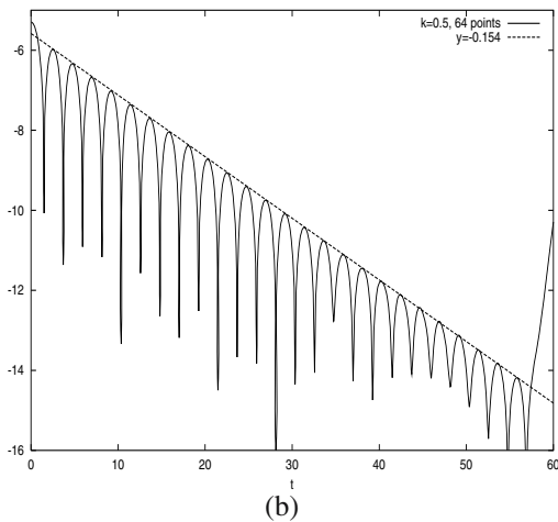
Fig. 2. Electric energy as a function of time for the linear Landau damping in the parallel case. (a) k=0.3 with N_x=N_v=64 points. (b) k=0.5 with N_x=N_v=64 points.
