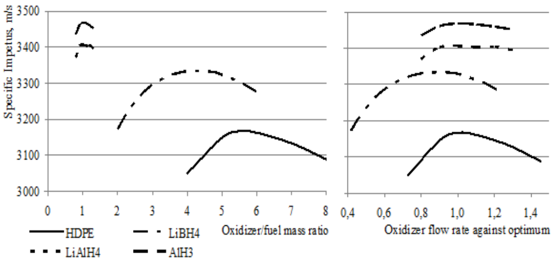
Pic. 1. Hydride-based propellant thermodynamic calculation results
