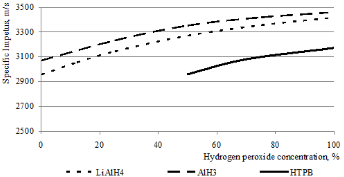
Pic. 2. Performance of hydrides with hydrogen peroxide
